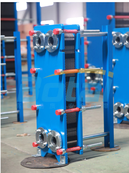
Detachable plate heat exchanger-M6B-1
