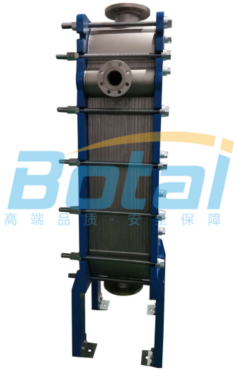
Fully welded plate and frame heat exchanger
