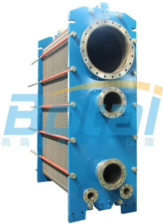
Plate condenser
